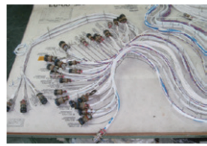
Wiring harnesses
